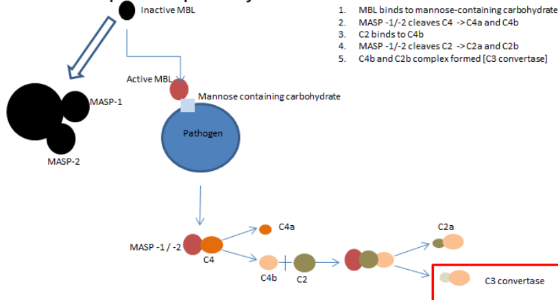
Fig 2. The lectin complement pathway
